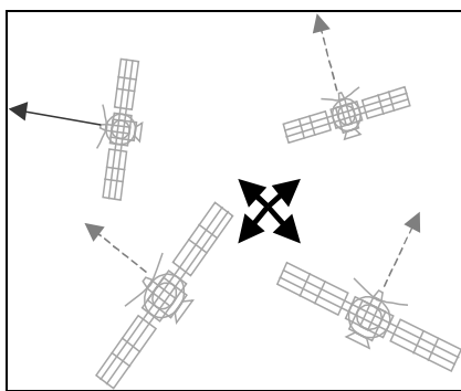
Fig. 10.Coordinatedplanning,eachspacecraftsensesa partoftheskyandprovidepossiblefutureplans
